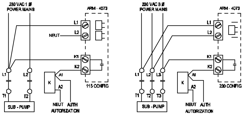
FIG 1 - Schematic 1595 - 009
